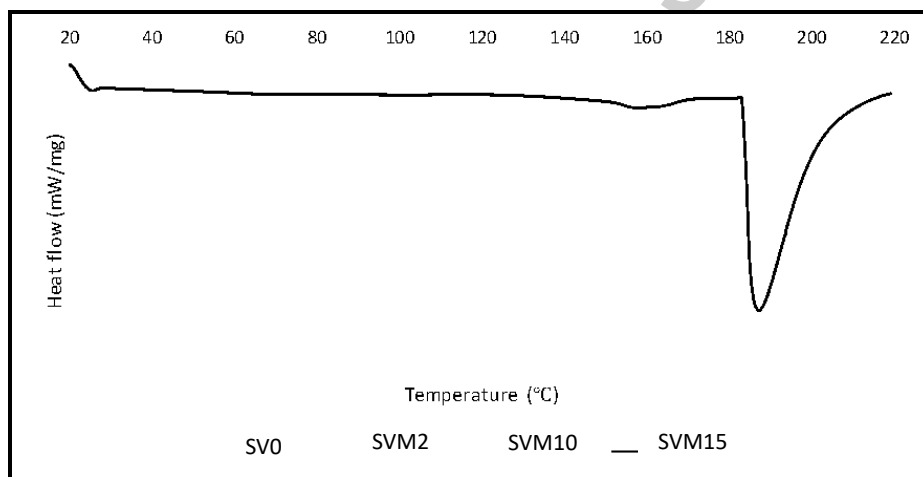
Figure 3. DSC thermogram of the membranes
