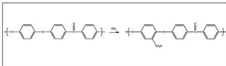
Figure 4. Process of PEEK sulfonation [23]
