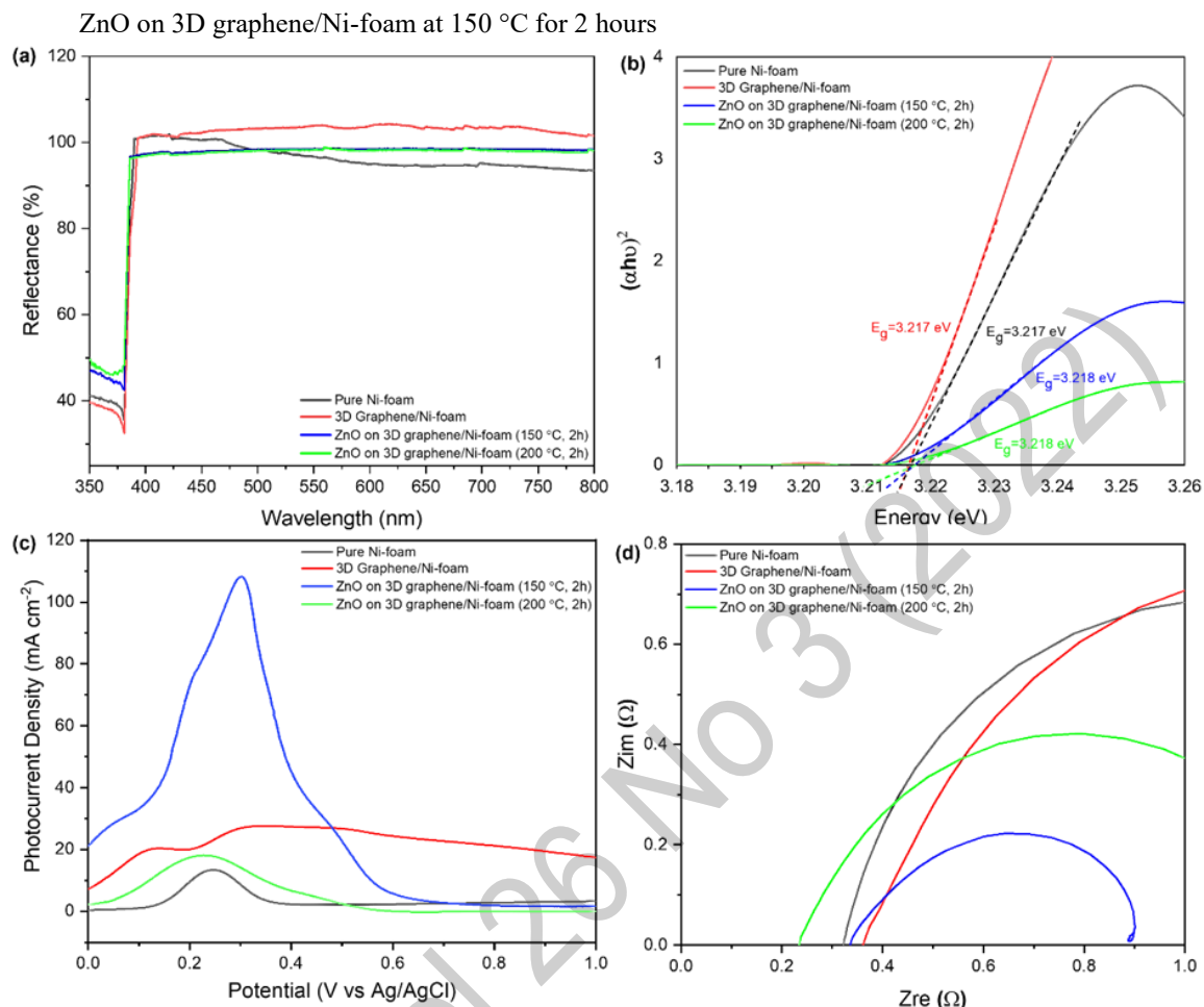
Figure 4. (a) Diffuse reflectance spectra, (b) Kubelka-Munk plot, (c) Photocurrent density at 0.0 – 1.0 V vs Ag/AgCl and (d) EIS analysis using Nyquist plot for pure Ni-foam, 3D graphene/Ni-foam, ZnO on 3D graphene/Ni-foam at 150 °C and 200 °C for 2 hours
