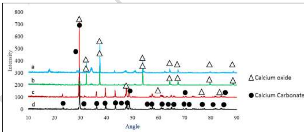
Figure 4. XRD patterns of a) industrial CaO, b) ESP T 900-3 , c) ESP T 700-3 , and d) RESP
