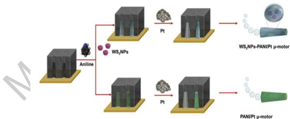
Figure 3. Schematic representation of \text{WS}_2\text{NPs-PANI}/\text{Pt} \mu -motor fabrication process. Reproduced with permission from ACS [40].
