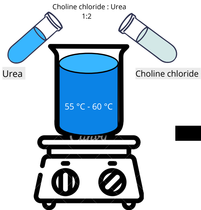
Preparation of Deep Eutectic Solvent: Reline
