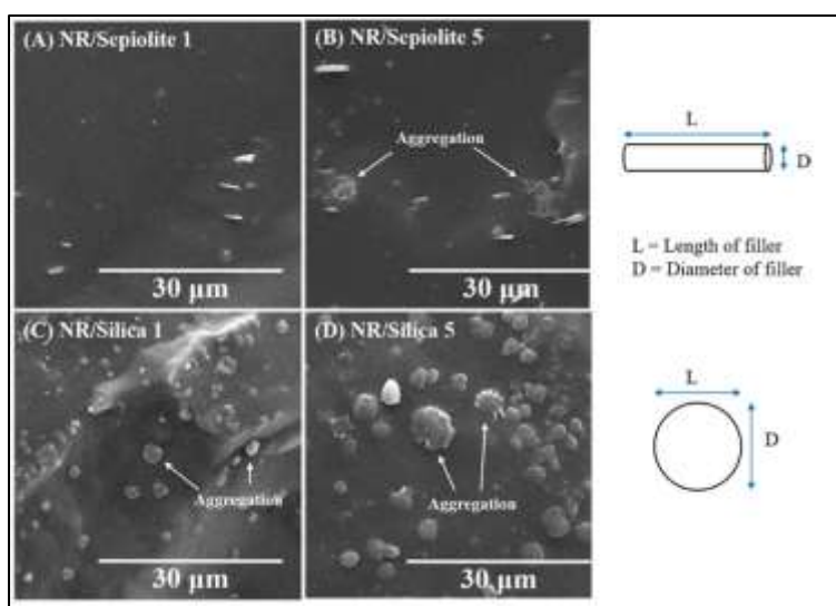
Figure 10. SEM micrographs of NR composites: (a) NR/Sepiolite 1 phr, (b) NR/Sepiolite 5 phr, (c) NR/Silica 1 phr, and (d) NR/Silica 5 phr at 500x
