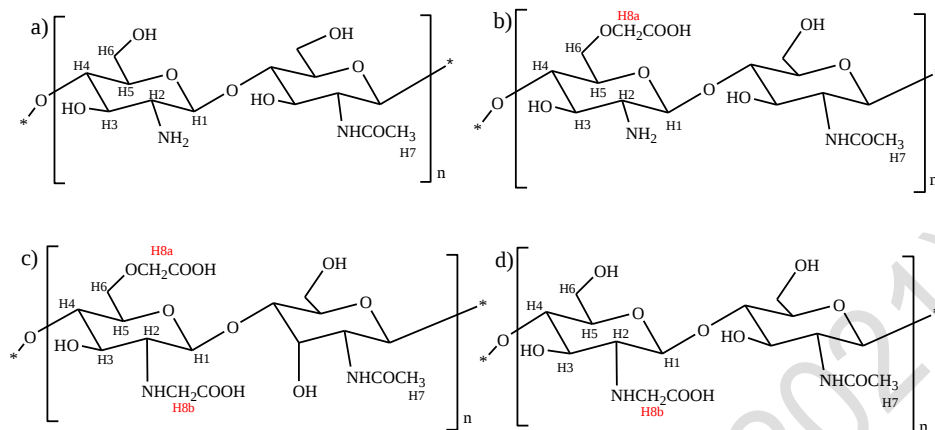
Figure 4. The chemical structure of a) chitosan b) O-CMC, c) N,O-CMC and d) N-CMC
