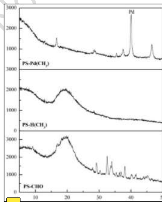
Figure 3. PXRD spectra of synthesized compounds
