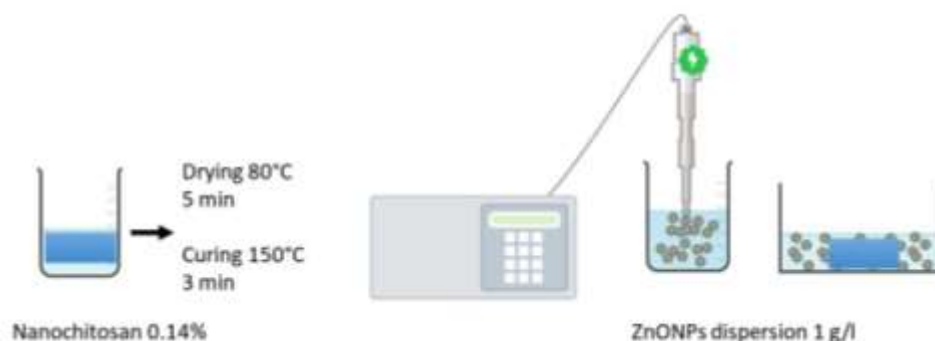
Figure 2. Coating process
