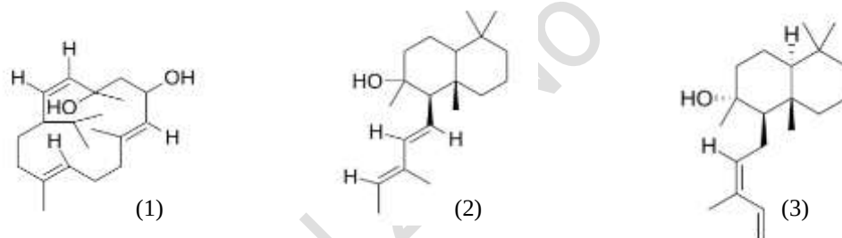
Figure 3. Chemical structure of (1) 4,8,13-cyclotetradecatriene-1,3-diol, (2) (11E,13Z)-labdadien-8-ol, (3) (12Z)-abienol
