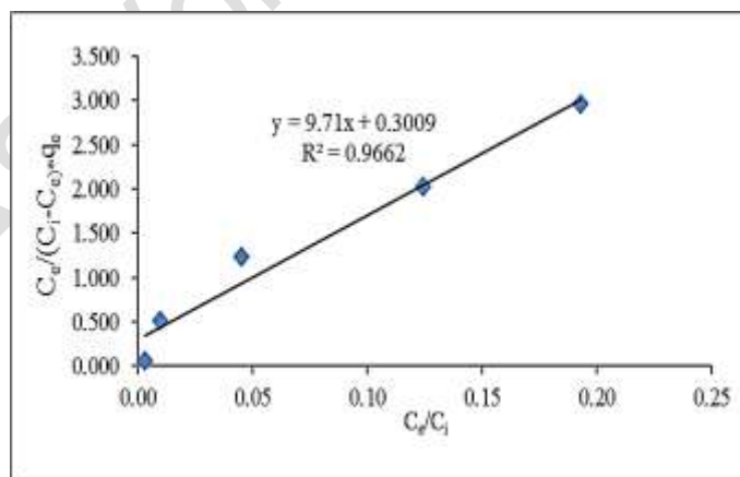
Figure 4. BET sorption isotherm of Mg^{2+}
