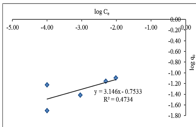
Figure 6. Freundlich sorption isotherm of Mg^{2+}
