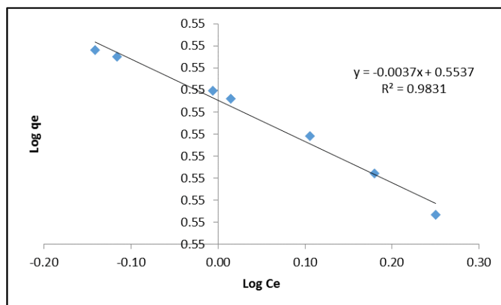
Figure 7. Freundlich sorption isotherm of Ca^{2+}
