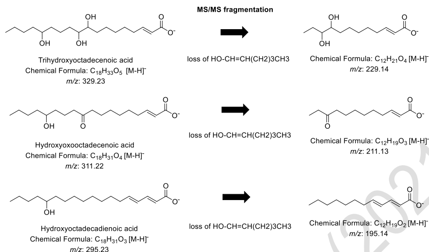
Figure 4. Proposed MS/MS fragmentation of peaks 4, 6 and 8 with the neutral loss of 100 atomic mass unit (amu) corresponding to HO-CH=CH(CH_2)_3CH_3 moiety
