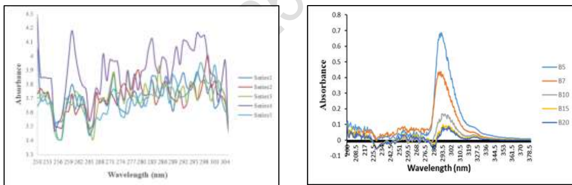
Figure 3. a) UV-Vis absorbance for unsaturated fatty acids b) UV-Vis absorbance spectra for saturated fatty acid
