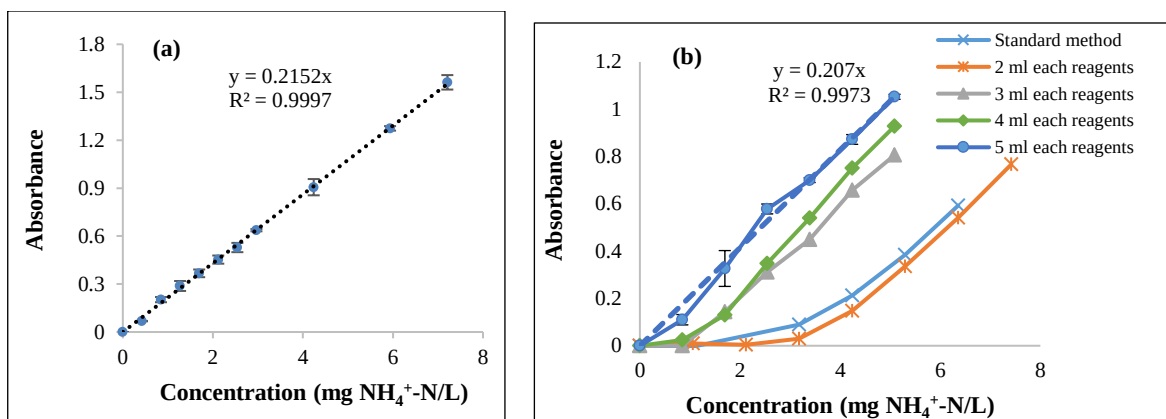
Figure 2. Relationship between the concentration and absorbance for \text{NH}_4^+\text{-N} determination: (a) using distilled water, and (b) using mineral medium with varying the amount of reagents
