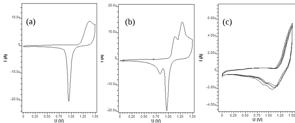
Figure 1. Voltammograms of electrochemical behavior for gold electrode by cyclic voltammetry in 0.5 M \text{H}_2\text{SO}_4 ; (a) clean surface, (b) presence of multilayer of oxides at the surface and (c) the passivating layer covered the electrode surface
