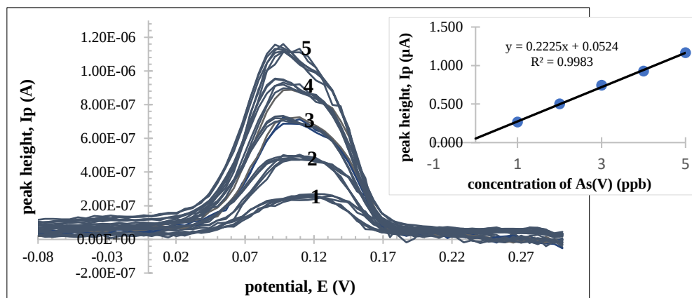
Figure 3. DPASV voltammogram and linear curve of I_p against concentration of As(V) standard additions: 0.4 mL of As(V) 50 ppb in 2 M HCl at 1: first addition, 2: second addition, 3: third addition, 4: fourth addition and 5: fifth addition ( n = 6 )
