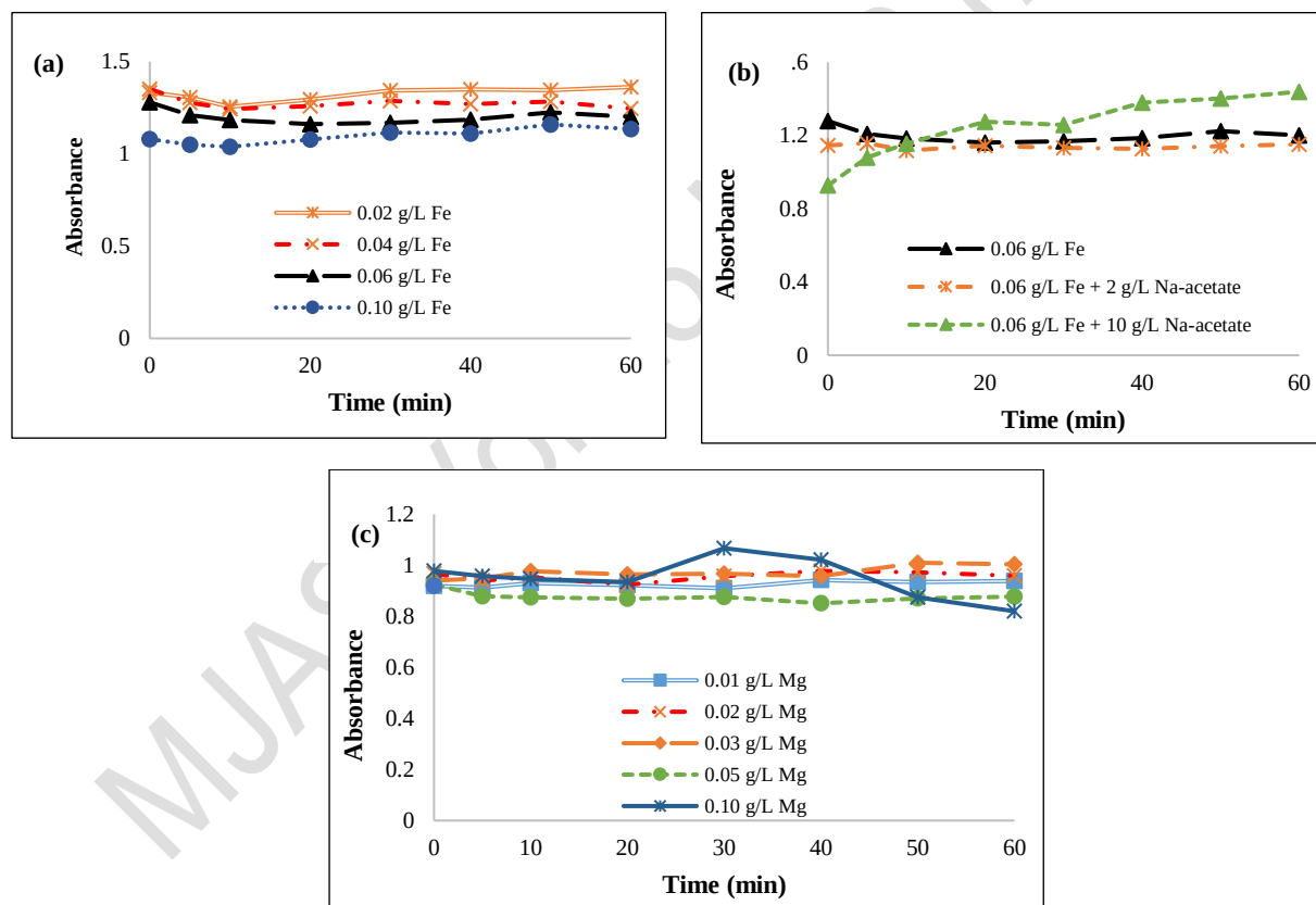
Figure 3. UV-Spectrophotometer absorbance of 5 \text{ mg/L NH}_4^+\text{-N} in mineral medium as per Figure 1 but varying: (a) \text{Fe}^{2+} concentration, (b) sodium acetate, and (c) \text{Mg}^{2+} concentration
