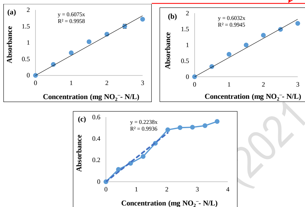
Figure 4. Calibration curves of \text{NO}_2^- - N using sulphanilamide method; standard was made with: (a) distilled water, (b) mineral medium, (c) mineral medium and 5 g/L sodium acetate
