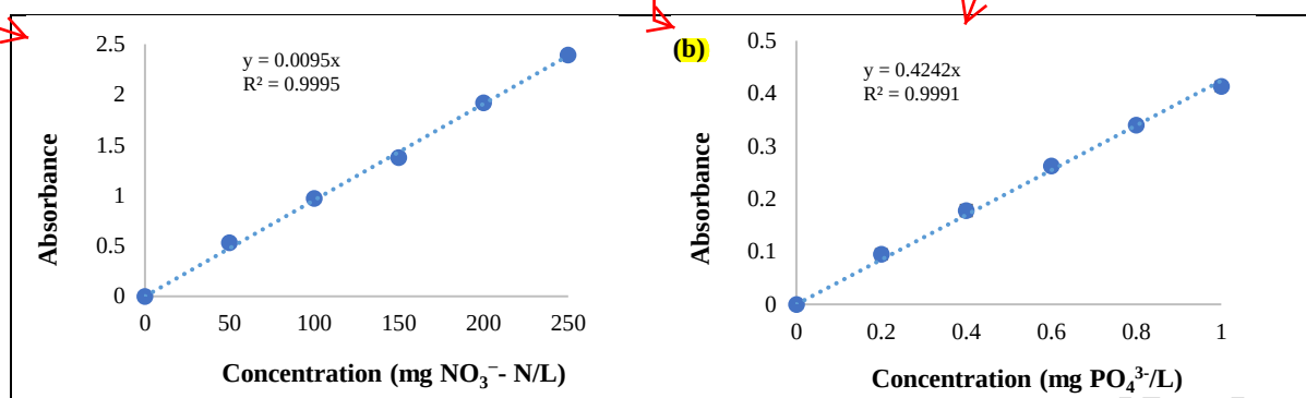
Figure 7. Calibration curves of \text{NO}_3^- -N and \text{PO}_4^{3-} . Standard was made with: (a) distilled water, and (b) mineral medium and 5 g/L sodium acetate
