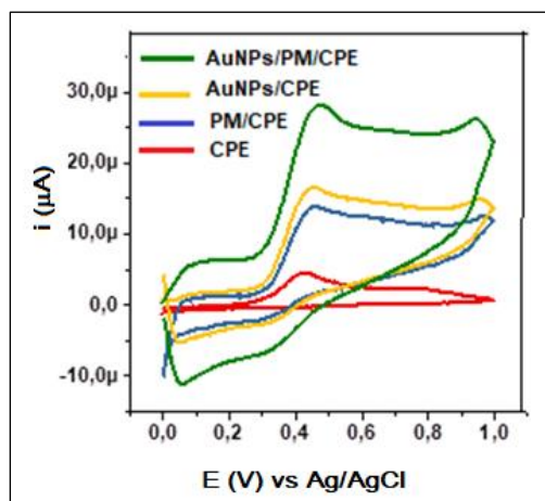
Figure 1. Cyclic 3 \mu M UA voltammogram in the scan rate of 100 mV/s using various electrodes
