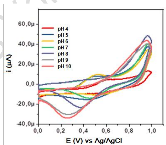
Figure 2. Cyclic voltammograms of 2 \mu M UA with pH variation using PBS with scan rate of 100 mV/s
