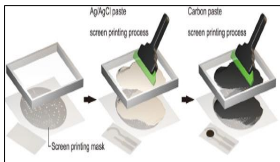
Figure 3. Schematic diagram on the fabrication of potentiometric pH sensor
