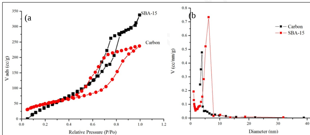
Figure 2. N 2 adsorption-desorption isotherm (a) and pore size distribution (b) of activated nanoarrays carbon (AONC-1h) and SBA-15
