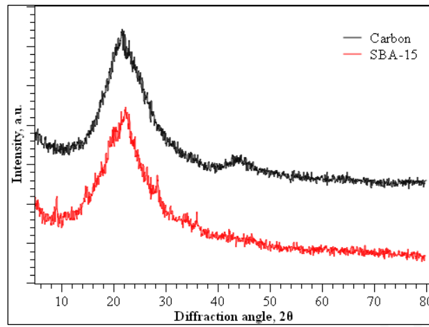
Figure 1. XRD analysis of SBA-15 and activated nanoarrays carbon
