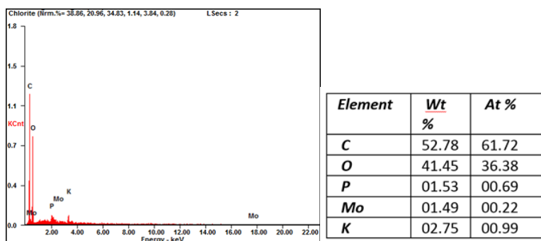
Figure 5. EDX analysis of ordered nanoarrays activated carbon
