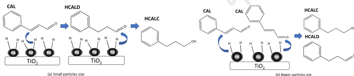
Figure 5. Schematic process of cinnamaldehyde hydrogenation on Pd/TiO 2 catalysts
