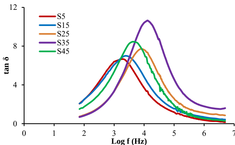
Figure 8. The frequency dependence of \tan \delta for PEO-GO- \text{NH}_4\text{CF}_3\text{SO}_3 salted system at room temperature
