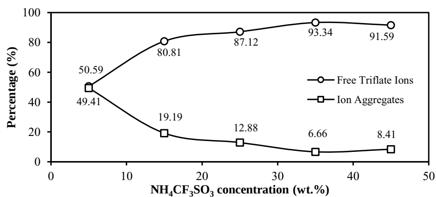
Figure 4. Percentage of free triflate ion and ion aggregates of PEO-GO-NH 4 CF 3 SO 3 salted system
