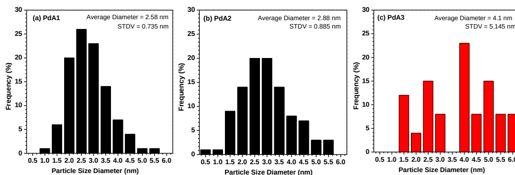
Figure 3. Particle size histogram for the Pd/TiO 2 catalysts prepared at different temperatures; a) 1 °C, b) 25 °C, and c) 50 °C
