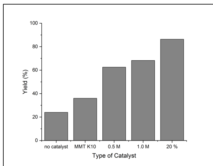
Figure 7. Percentage of FAME yield at 6 hours reaction period, 12:1 methanol to oil molar ratio and 4% w/w
