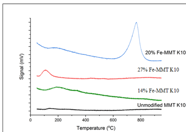
Figure 5. Peak of acidity of montmorillonite K10 and its modifications from TPD- \text{NH}_3 analysis
