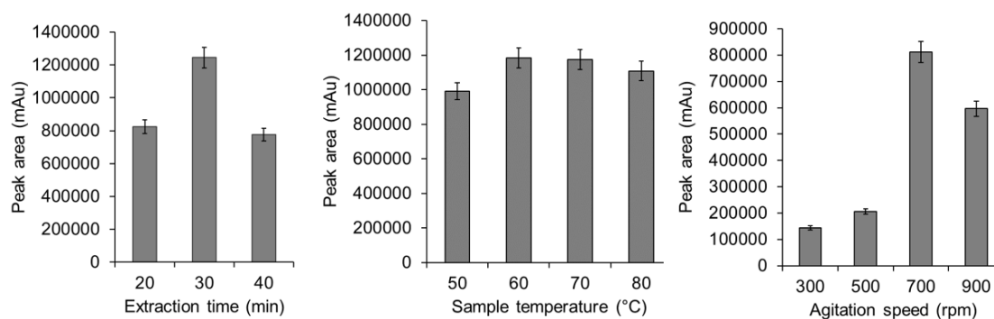
Figure 2. Effect of extraction time (a), sample temperature (b) and agitation speed (c) on the extraction efficiency of HS-MP-LPME for the extraction of PHE in spiked deionized water
