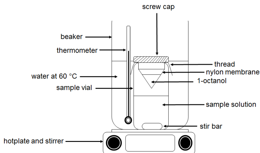
Figure 1. Schematic of headspace membrane-protected liquid phase microextraction
