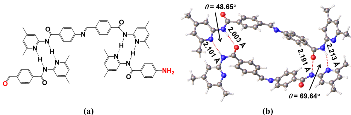
Figure 5. The chemical structure of the ternary complex (a) and the DFT optimised [B3LYP/6-311G(d,p)] duplex complex (b) involving the formation of imine 7 . The former assumes only the \text{N-H}\cdots\text{N} intermolecular hydrogen bonding, while the latter participates in a reciprocal interaction via \text{N-H}\cdots\text{N} and \text{N-H}\cdots\text{O}
