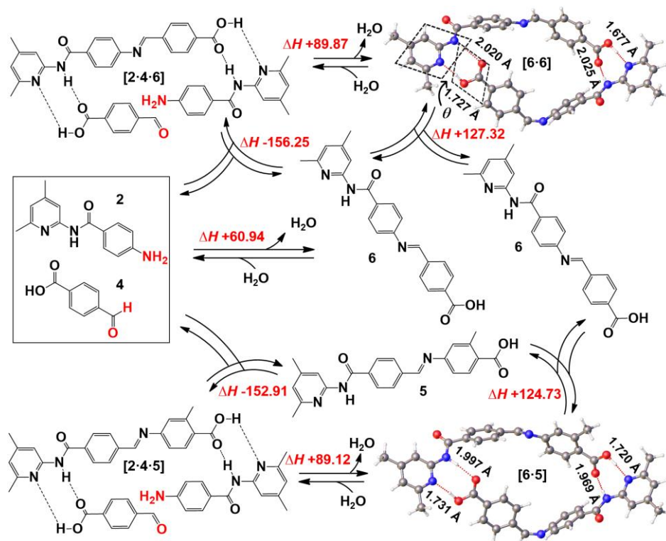
Figure 4. The formation of imine 6 via direct condensation of 2 and 4 , as well as through thermodynamically [\Delta H (kJ/mol)] favourable autocatalytic cycles mediated by ternary complexes [2·4·6] or [2·4·5] . The optimised [B3LYP/6-311G(d,p)] duplex complexes [6·6] and [6·5] are shown along with the measured intermolecular hydrogen bond (red dotted lines) lengths. The angle, \theta represents the degree of deviation between the mean planes of the amidopyridines and carboxylic acids
