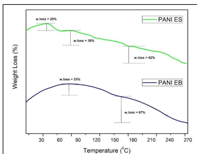
Figure 3. TGA thermograms of PANI-EB and PANI-ES powder
