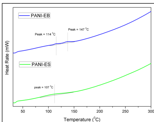
Figure 4. DSC thermogram of PANI-EB and PANI-ES powder
