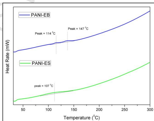
Figure 4. DSC thermogram of PANI-EB and PANI-ES powder
