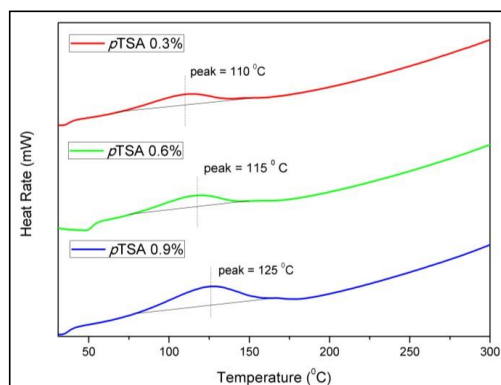
Figure 5. DSC thermogram of doped PANI-ES powder with varying concentrations of p TSA (0.3, 0.6, and 0.9 wt.%)
