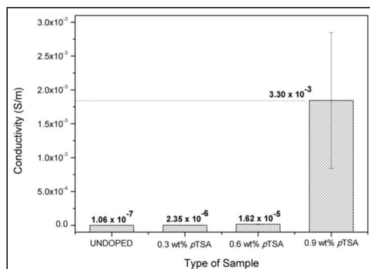
Figure 6. Conductivity of PANI cotton fabrics at different weight percentage of pTSA
