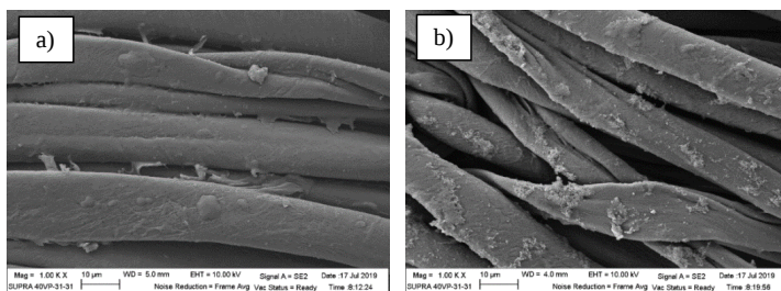
Figure 2. Field emission scanning electron microscope (FESEM) micrographs of (a) bare cotton fabric (b) cotton fabric doped with 0.9 wt% of PANI- p TSA
