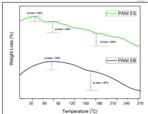
Figure 3. TGA thermograms of PANI-EB and PANI-ES powder
