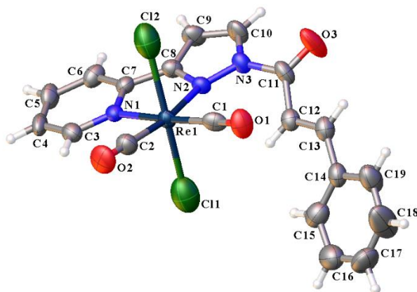
Figure 3. The X-ray crystallographic structure of \text{Re}(\text{CO})_2(\text{CnPyPz})\text{Cl}_2 complex with displacement ellipsoids drawn at the 50% probability level CCDC Num. 1978548
