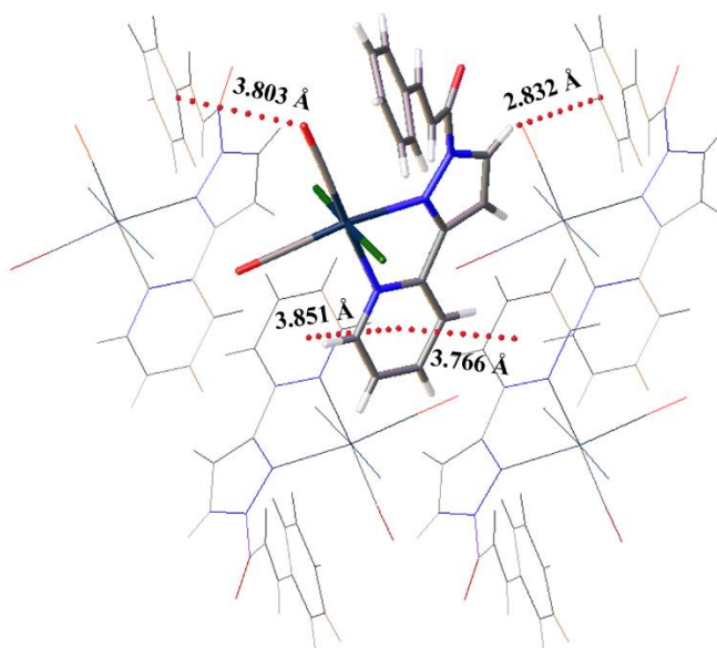
Figure 6. The intermolecular connections involving pyridine and benzene rings, namely \pi-\pi , \text{C}-\text{H}\cdots\pi and \text{C}=\text{O}\cdots\pi interactions
