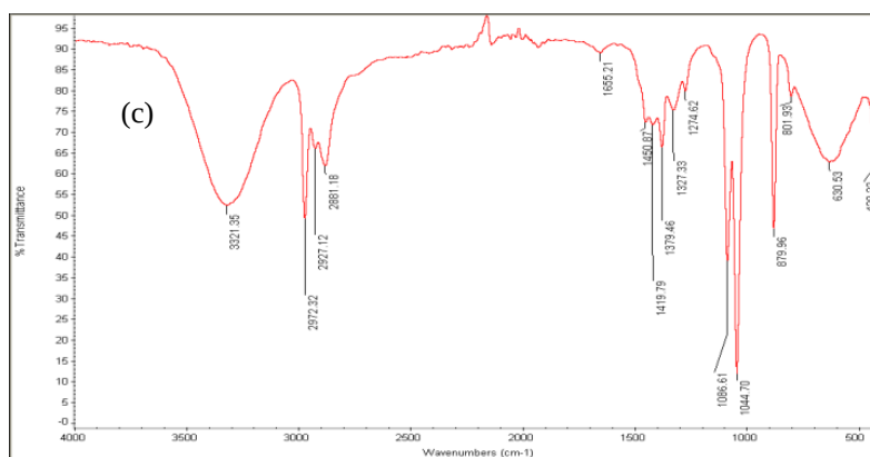
Figure 3. The IR spectra of P. amaryllifolius essential oils from (a) Kedah, (b) Selangor, and (c) Johor.
