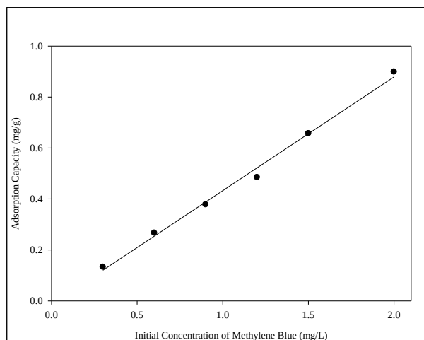
Figure 4. Effect of initial dye concentration on methylene blue sorption by N,O-CMCTS
