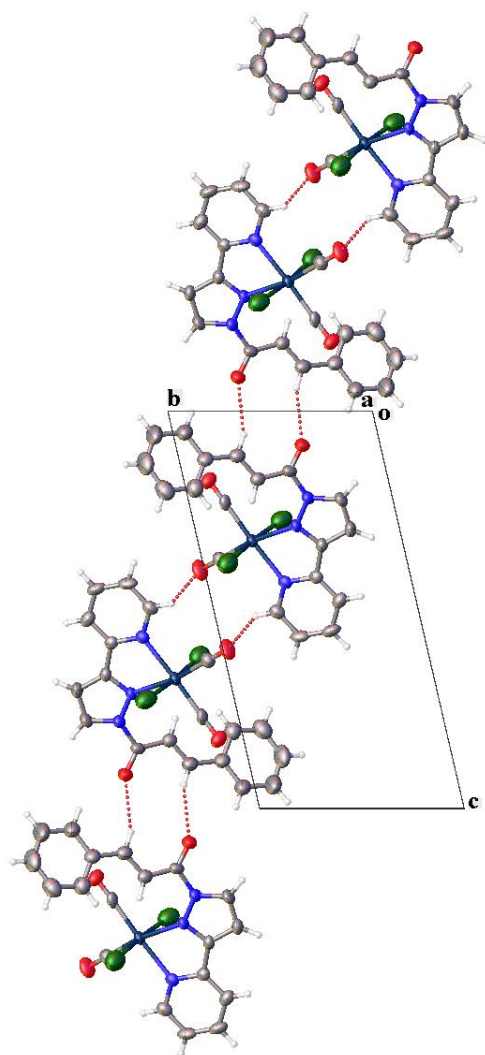
Figure 4. A partial view of the crystal packing of \text{Re}(\text{CO})_2(\text{CnPyPz})\text{Cl}_2 complex, illustrating one-dimensional chain viewed from a -axis
