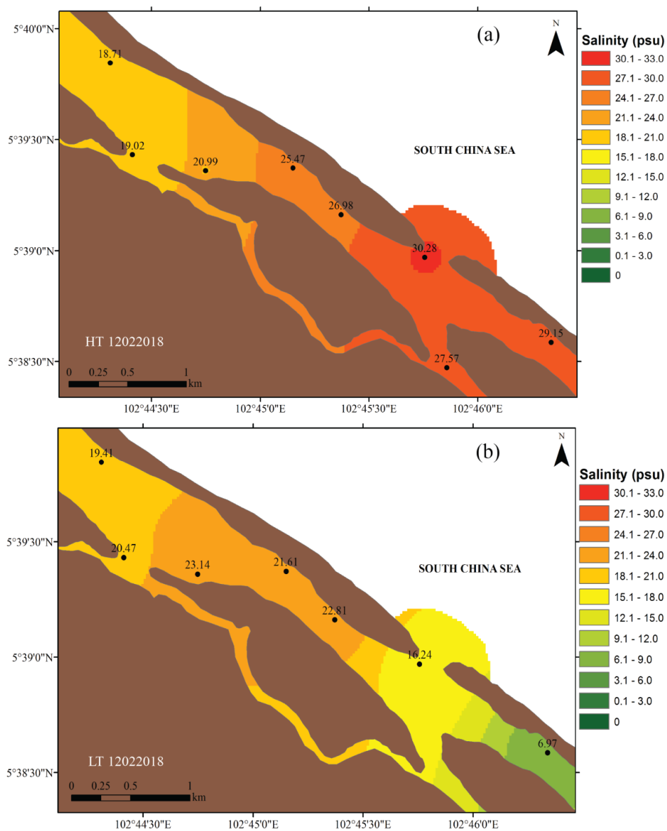
Figure 7. Salinity distribution in Setiu Lagoon during (a) high and (b) low tides on 12 February 2018
