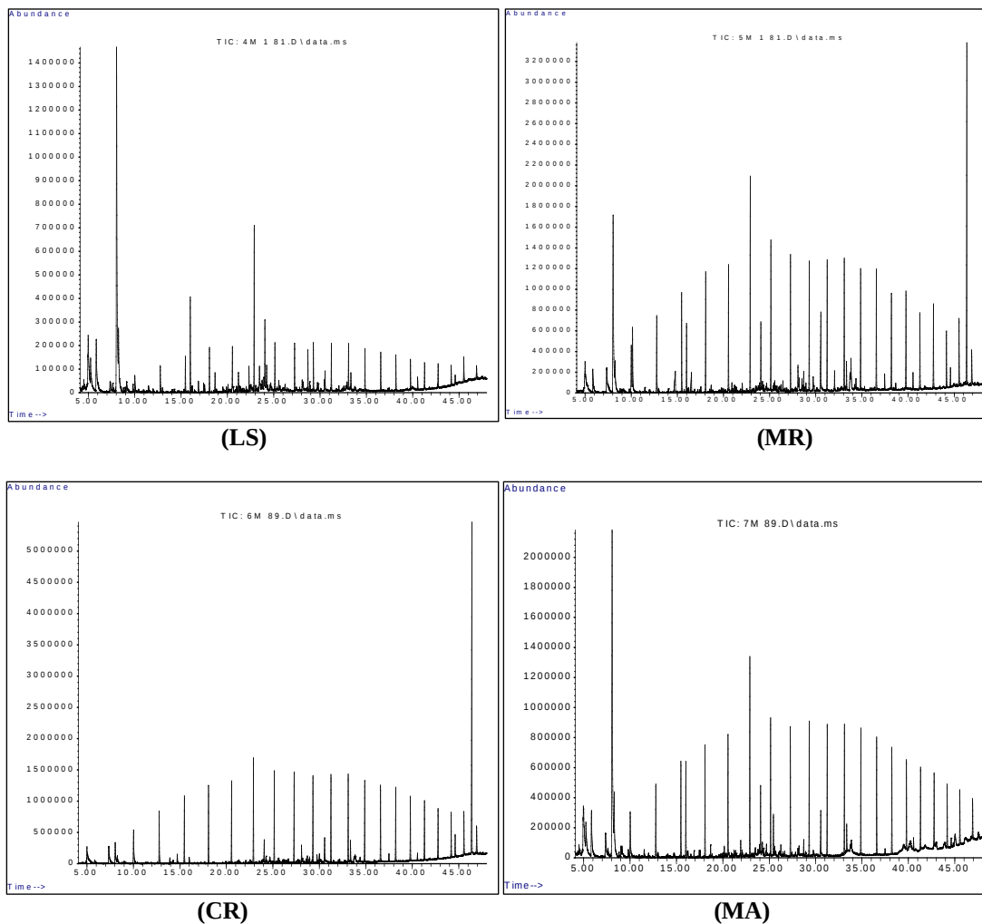
(LS) (MR) (CR) (MA) Figure 2. Total ion chromatogram of DCM extracts of dried MR , CR , and MA with n-alkanes
