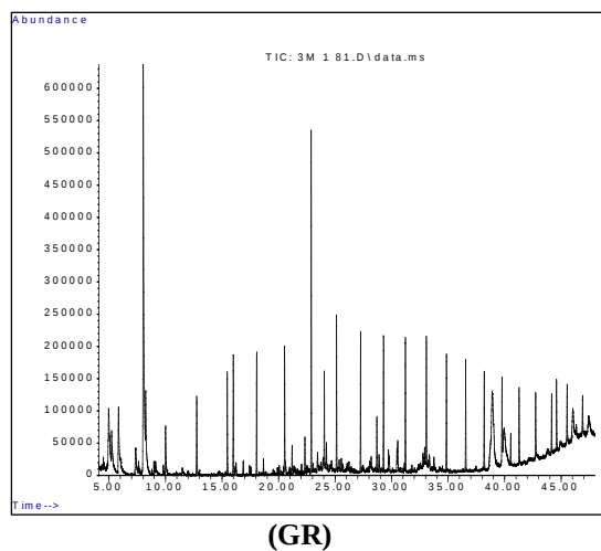
(GR) Figure 1. Total ion chromatogram of DCM extracts of dried PB , HP and GR with n-alkanes
