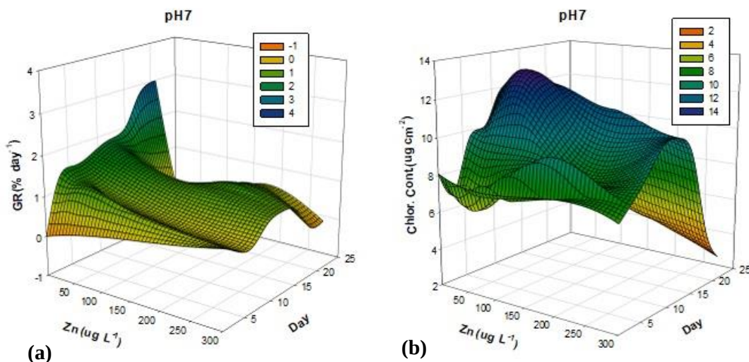
Figure 6. The (a) growth rate (GR, %), and (b) chlorophyll content of P. boryana cultured for 21 days at pH 7
