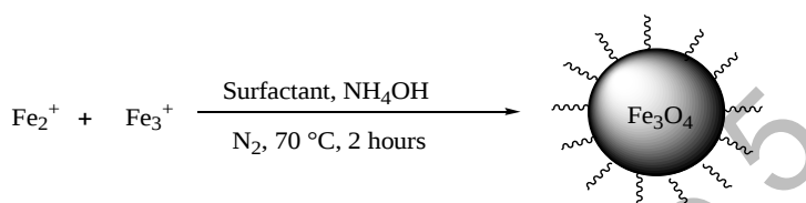
Scheme 1. Preparation of surfactant-bound Fe 3 O 4 nanoparticles
