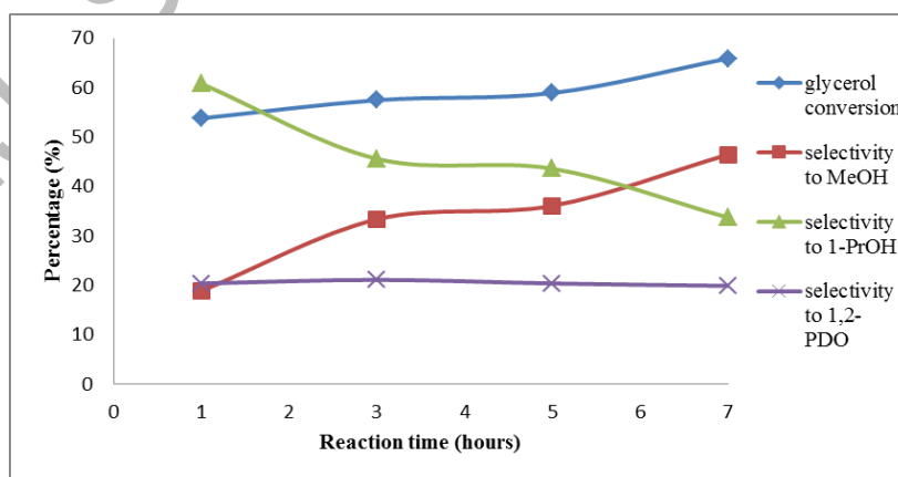
Figure 8. Catalytic profile effect of reaction time at 170 °C
