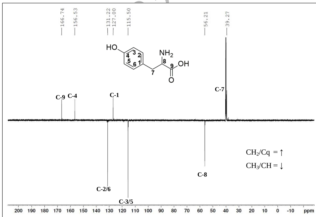
Figure 14. The NMR-APT (DMSO, 175MHz) Spectrum of L-Tyrosine (5)
