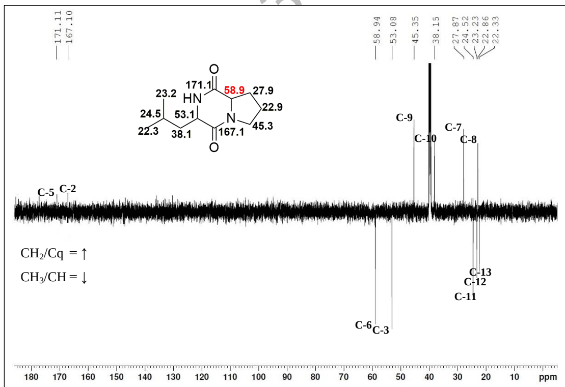
Figure 11. The NMR-APT (DMSO, 175 MHz) Spectrum of (+)Cyclo(-Tyr-Leu) (4)
