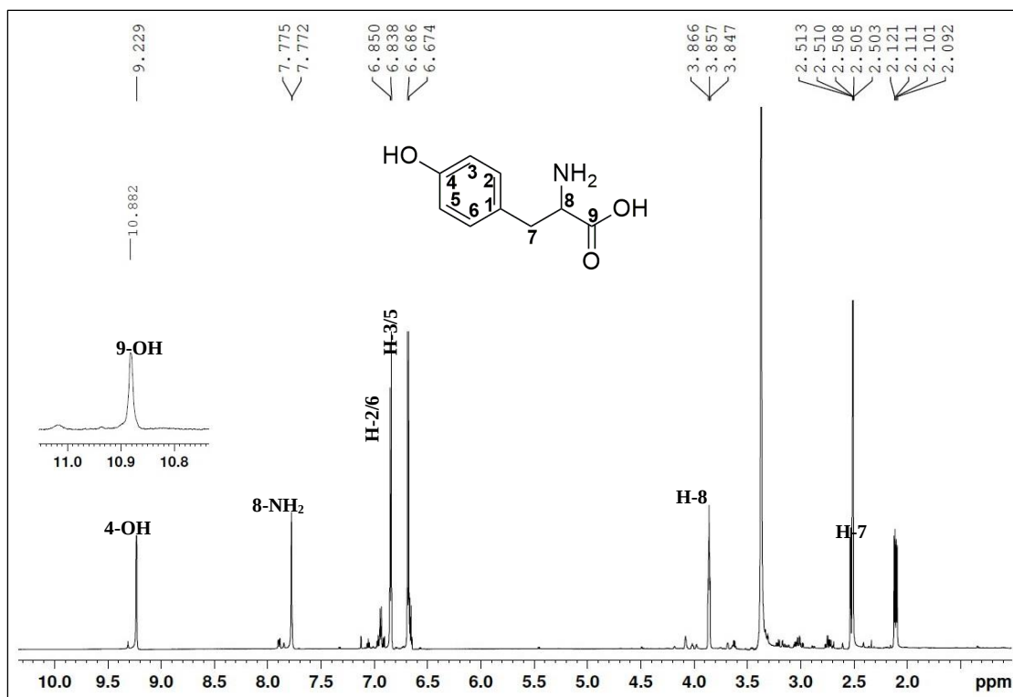
Figure 13. The 1 H-NMR (DMSO, 700 MHz) Spectrum of L-Tyrosine (5)
