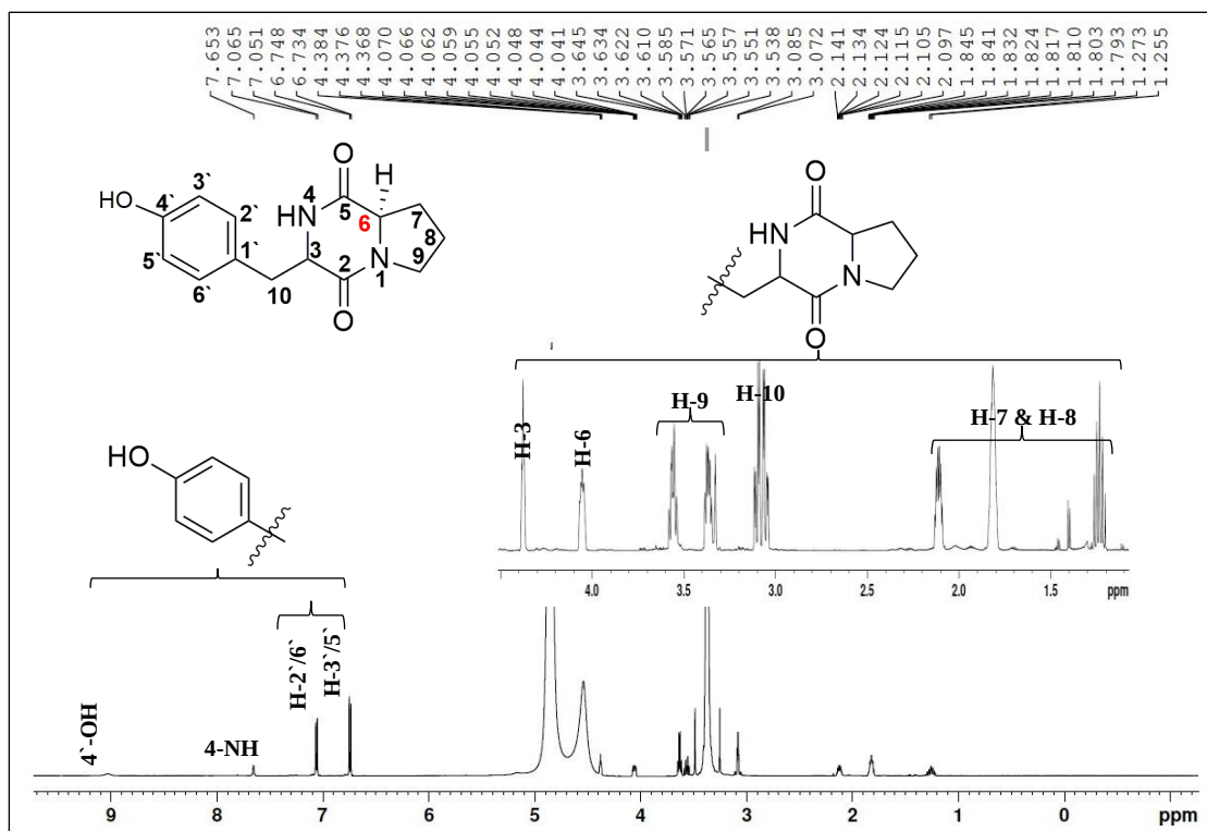
Figure 4. The 1 H-NMR (CD 3 OD, 700 MHz) Spectrum of (-)-Cyclo(-Pro-Tyr) (2)
