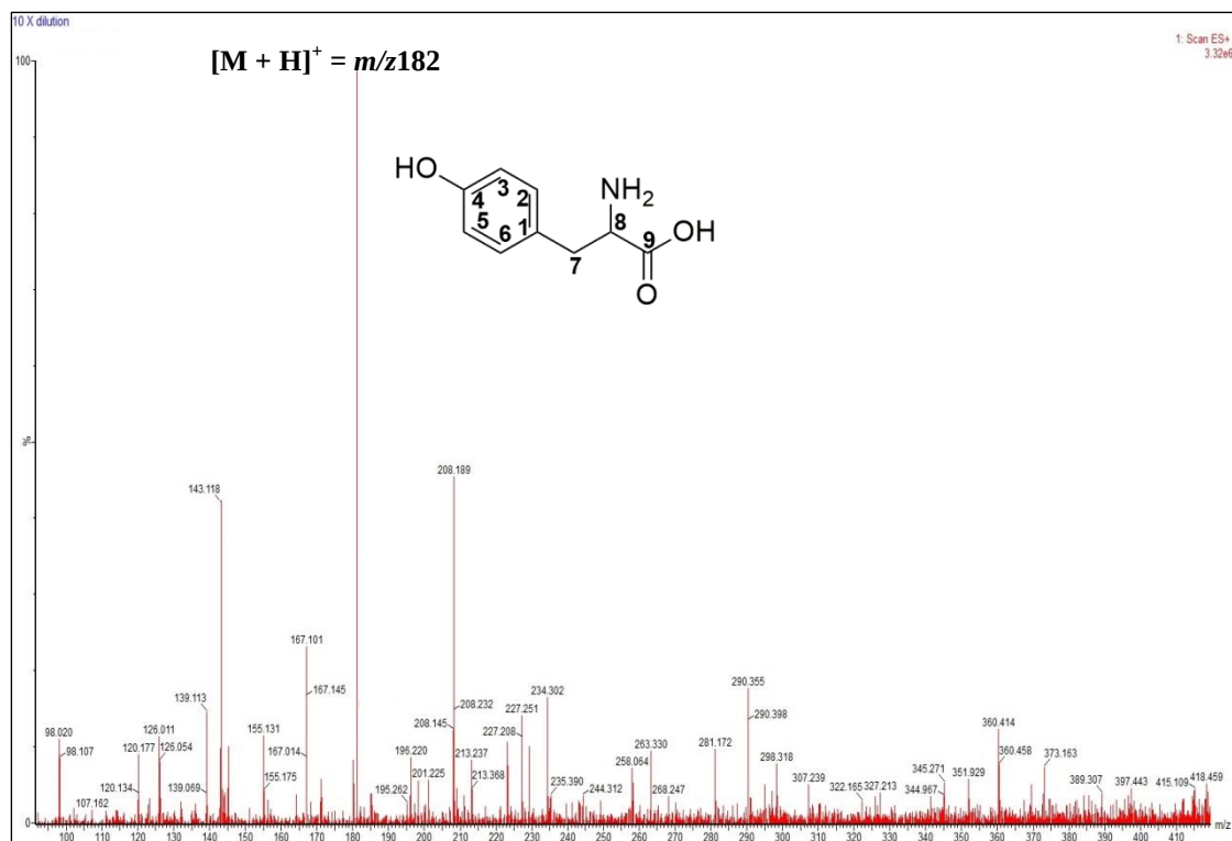
Figure 15. The LC-MS Spectrum of L-Tyrosine (5)
