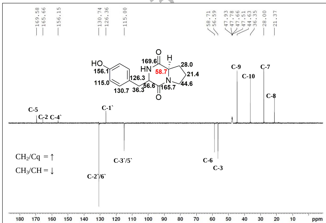
Figure 5. The NMR-APT(CD 3 OD, 175 MHz) Spectrum of (-)-Cyclo(-Pro-Tyr) (2)
