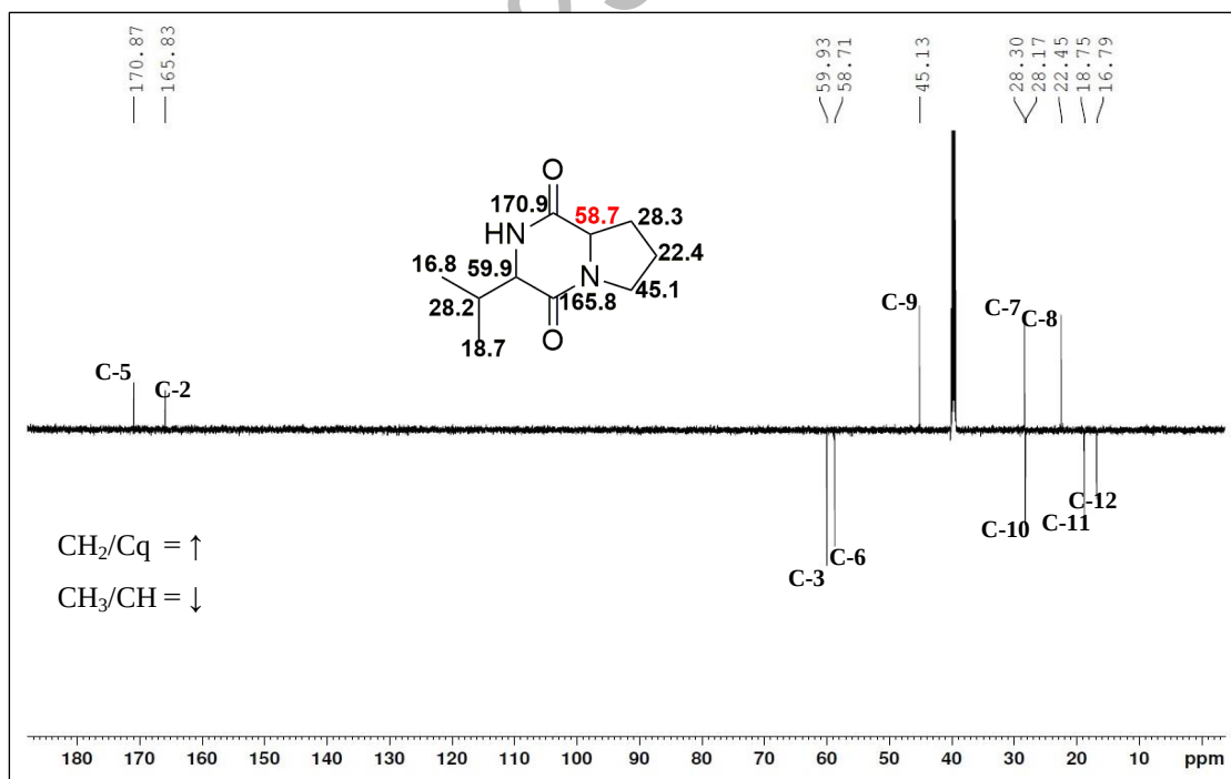
Figure 2. The 13 C NMR-APT (DMSO, 175 MHz) Spectrum of Cyclo(-Pro-Val) (1)
