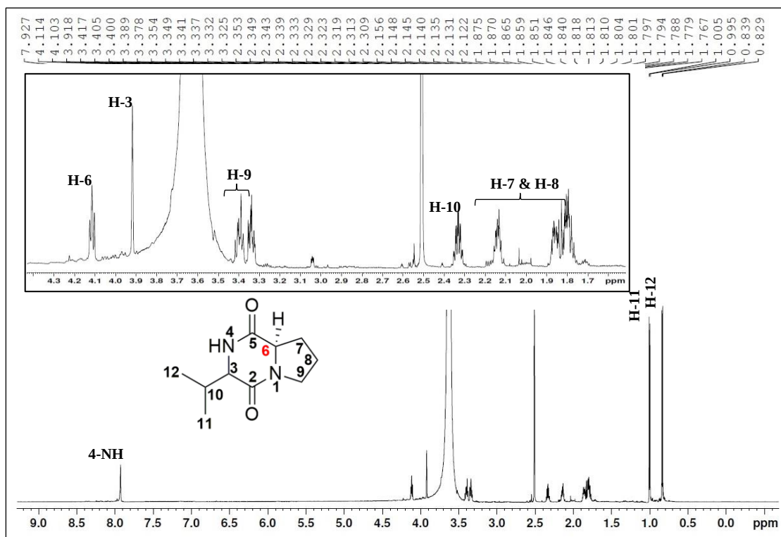
Figure 1. The 1 H-NMR (DMSO, 700 MHz) Spectrum of Cyclo(-Pro-Val) (1)
