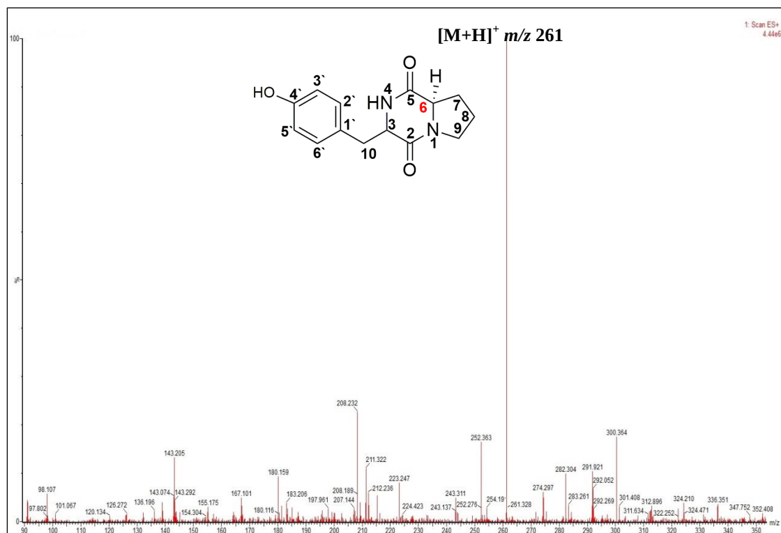
Figure 6. The LC-MS Spectrum of (-)-Cyclo(-Pro-Tyr) (2)
