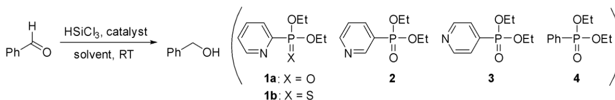
Figure 1. Hydrosilylation reaction of benzaldehyde
