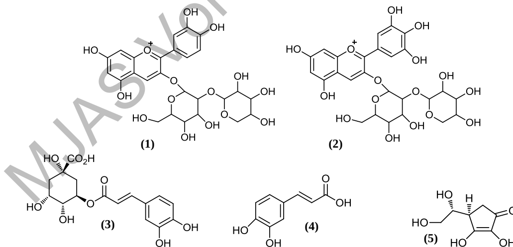
Figure 4. Proposed structures for the identified compounds in the H. sabdariffa water extract
