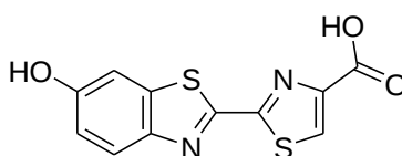
Figure 1. Chemical structure of D-luciferin
