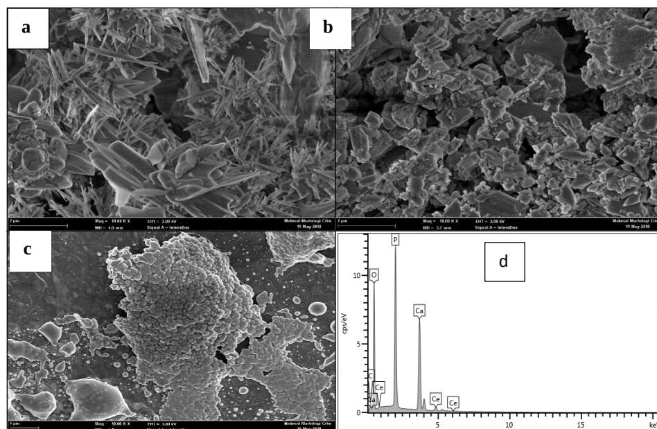
Figure 2. FESEM image for Ce/Ca (30:70)/AC catalysts calcined at (a) 500 °C, (b) 700 °C and (c) 1000 °C for 5 hours and (d) EDX result of Ce/Ca (30:70)/AC catalysts calcined at 500 °C
