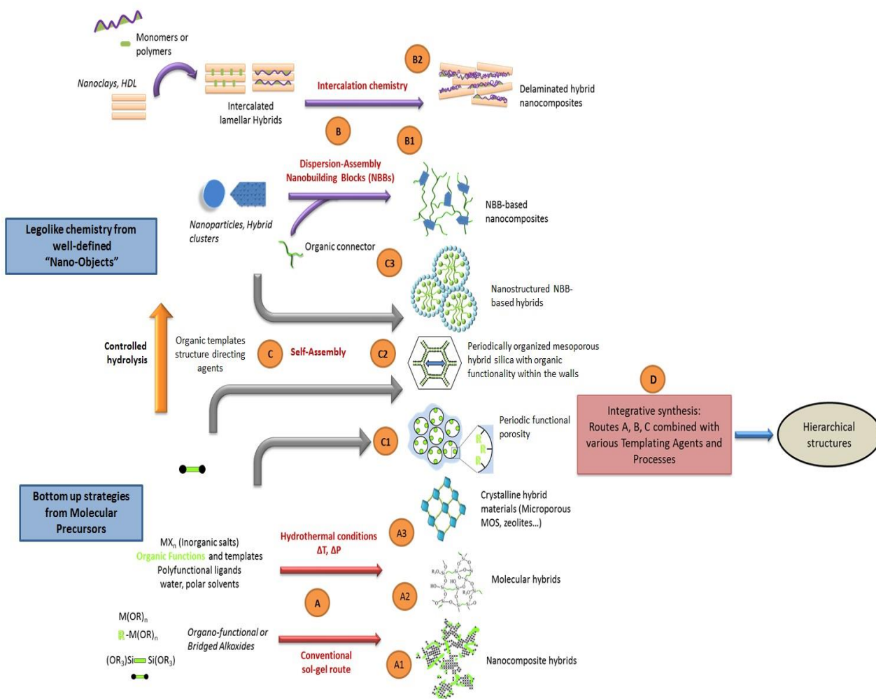
Figure 3. Main chemical routes for the synthesis of organic-inorganic hybrids
