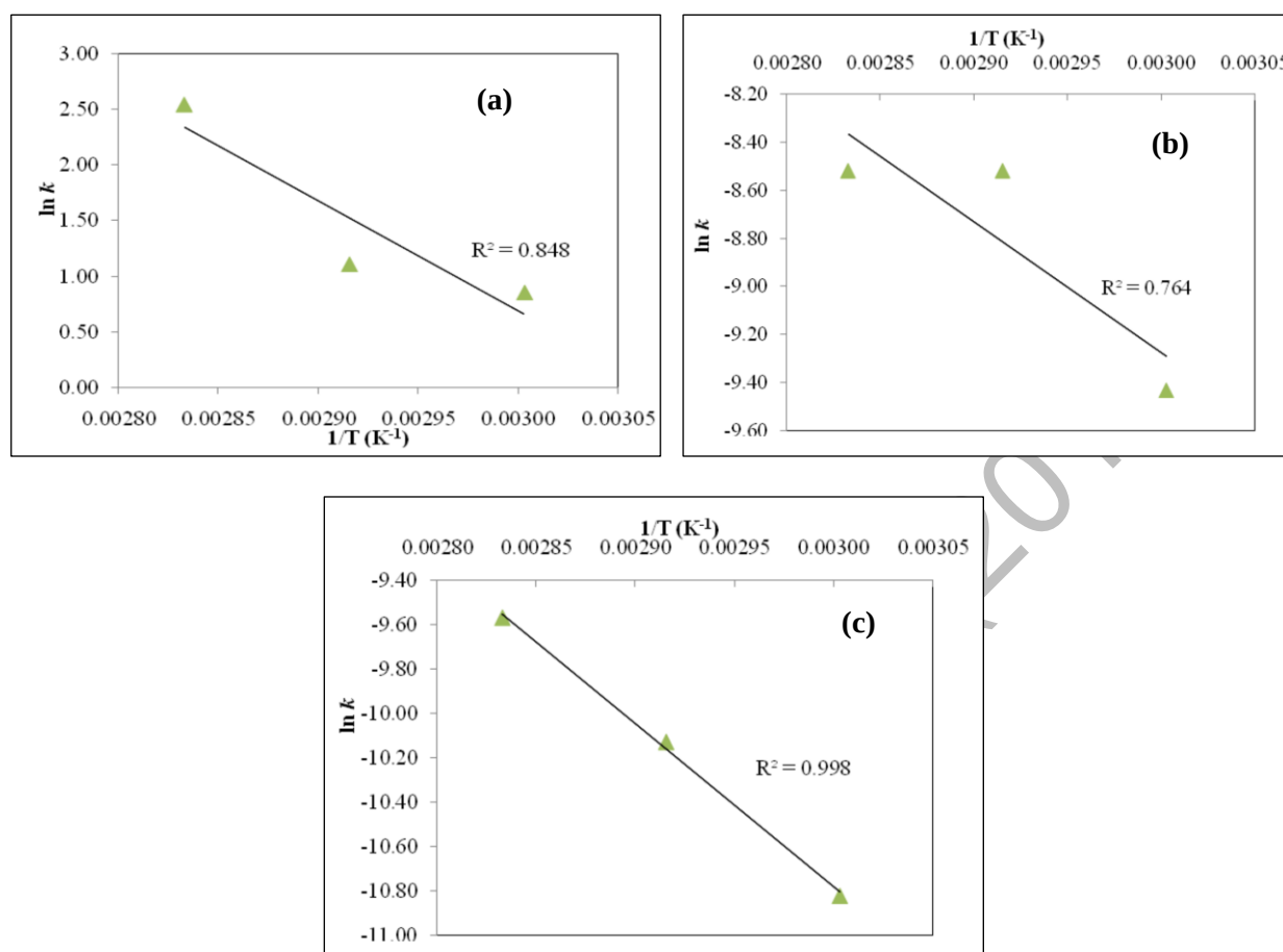
Figure 2. Arrhenius plots of (a) total phenolic content (b) DPPH radical scavenging activity and (c) XO activity in Yanang leaf extract
