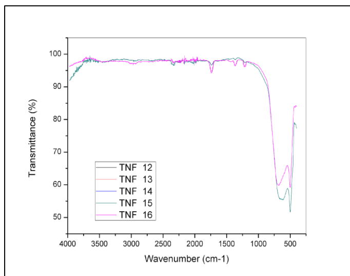
Figure 1. FTIR analysis of TNF sample after calcination process at 850\text{ }^{\circ}\text{C} for 2 hours
