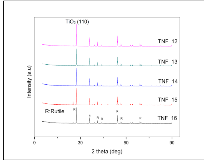
Figure 2. XRD patterns for TNF sample
