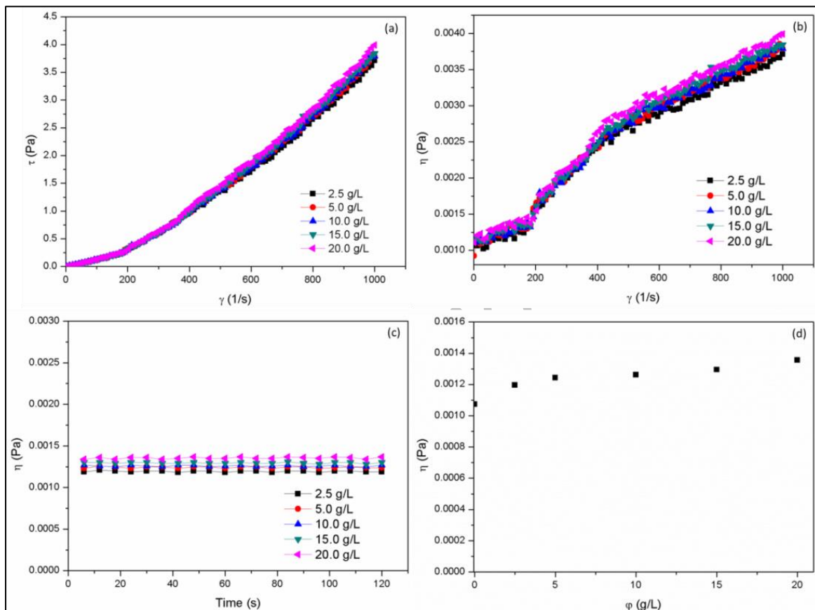
Figure 6. Rheological study (a) Shear stress versus shear rate, (b) Viscosity versus shear rate, (c) Viscosity versus time and (d) Viscosity versus \text{TiO}_2 concentration
