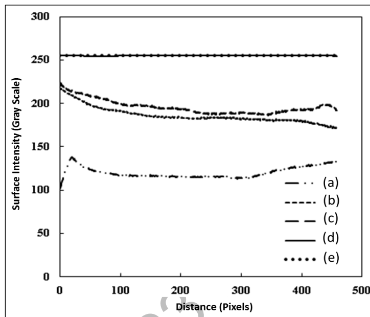
Figure 4. 2-D surface plotting for coating of different concentration (a) 2.5 g/L, (b) 5.0 g/L, (c) 10.0 g/L, (d) 15.0 g/L and (e) 20.0 g/L
