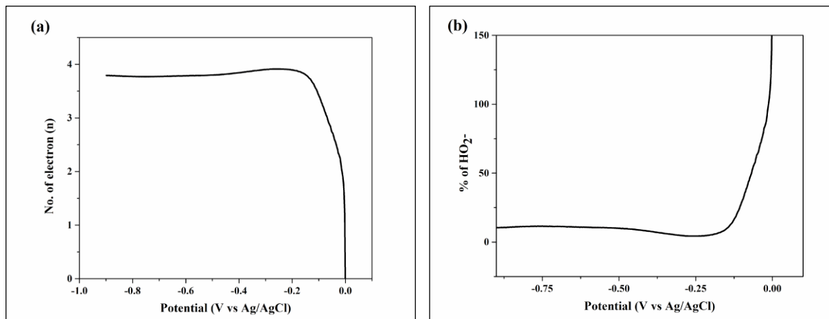
Figure 4. (a) Plot of electrons transfer number (n) vs potential and (b) % of \text{HO}_2^- vs potential for MWCNT/PTFE/Pt electrode.
