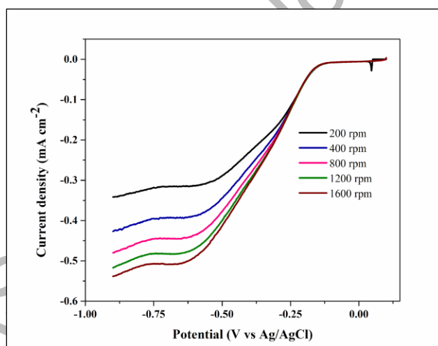
Figure 2. The ORR polarisation curves of MWCNT/PTFE/Pt electrodes in oxygen saturated environment of 0.1M KOH electrolyte with different rotation rate (scan rate: 10 mV s -1 )
