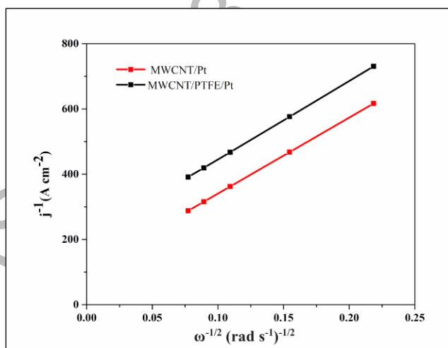
Figure 3. Koutecky-Levich (K-L) plots for MWCNT/Pt and MWCNT/PTFE/Pt electrodes
