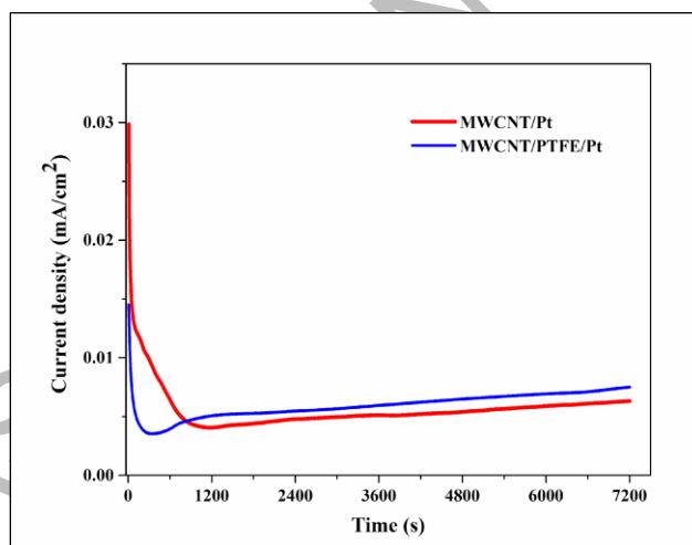
Figure 5. The chronoamperometric curves for synthesised catalyst in 0.1 KOH electrolyte solution at 0.3V
