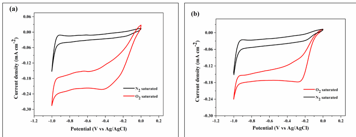
Figure 1. Cyclic voltammogram of (a) MWCNT/Pt and (b) MWCNT/PTFE/Pt electrodes in the O 2 and N 2 gas saturated of 0.1 M KOH electrolyte solution (scan rate: 10 mVs -1 )
