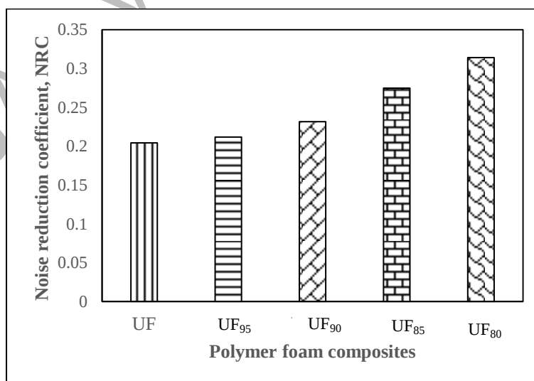
Figure 7. Noise reduction coefficient of polymer foam composites
